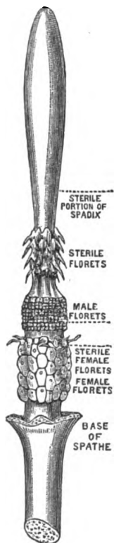
FIG. 236. — The spadix, with flowers, of an Arum; the large showy spathe is removed. (From Cavers.)
